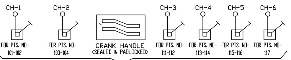
CRANK HANDLE KEYS (ELECTRICALLY INTERLOCKED WITH CONCERNED SIGNALS)
